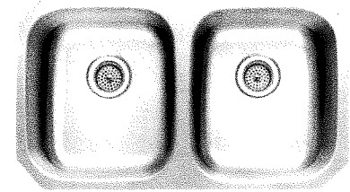
RUSTY @ $195 SIN-16-DBLBWL-5050-3218 Outside - 32½" x 18½" Left Inside - 14½" x 16½" Right Inside - 14½" x 16½" Depth - 9" Minimum Cabinet - 36"
