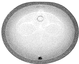
CLYDE @ $59 SIN-POR-UNDOVLWHT-1714 Outside - 19"x16" Inside - 17"x14" Depth - 8"
