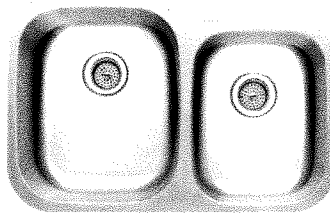
DUSTIN @ $195 SIN-16-DBLBWL-6040-3221 Outside - 32" x 20¾" Left Inside - 15¾" x 18¾" Right Inside - 13" x 16½" Depth - 9" x 7½" Minimum Cabinet - 36"
