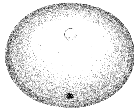
DUKE @ $59 SIN-POR-UNDOVLWHT-1512 Outside - 17"x14" Inside - 15"x12" Depth - 7½"
