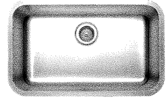
KATY @ $195 SIN-16-SINBWL-3118 Outside - 31½" x 18½" Inside - 29½" x 16¾" Depth - 9" Minimum Cabinet - 36"
