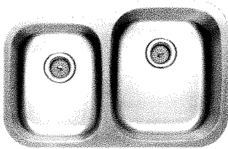
RAMBO @ $195 SIN-16-DBLBWL-4060-3221R Outside - 32" x 20¾" Left Inside - 13" x 16½" Right Inside - 15¾" x 18¾" Depth - 7½" x 9" Minimum Cabinet - 36"
